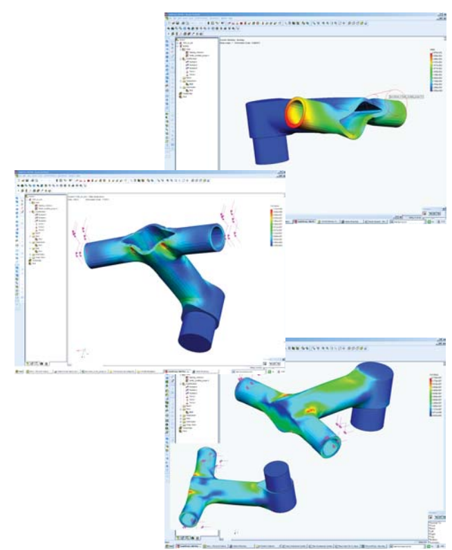
Left: views of the A-Bike in folded & unfolded positions, with Sir Clive Sinclair. Above: some FEA plots from the handlebar development process, simulating both static and fatigue stresses and deflections based on BS 6102, ISO 4210 and the JIS equivalents.
